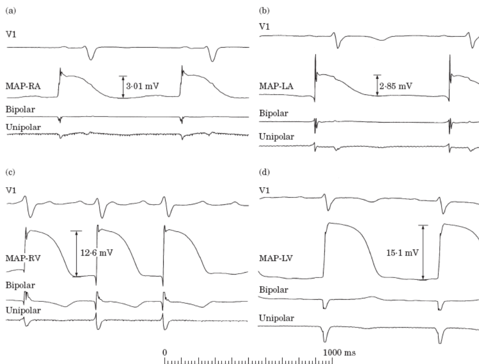
Fig. 13. Monophasic action potentials (MAPs) recorded using platinum-electrode ablation catheters from the right atrium (a), left atrium (b), right ventricle (c) and left ventricle (d) had characteristics consistent with those recorded using Ag-AgCl electrode catheters. Reproduced with permission from Yuan S, et al. (219).
