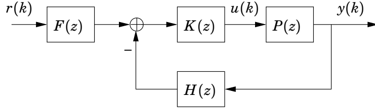
Figure 3 A standard feedback structure.
