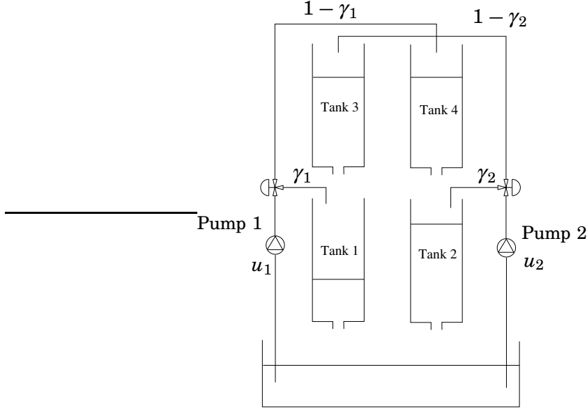
Figure 5 A schematic picture of the quadruple tank process
