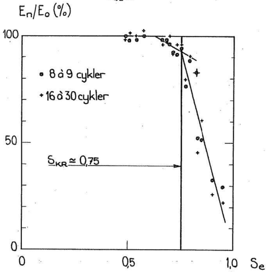
FIG 146 Material nr 14. Sarabondbruk vct=0,535. Cement mortar w/c-ratio=0,535.
