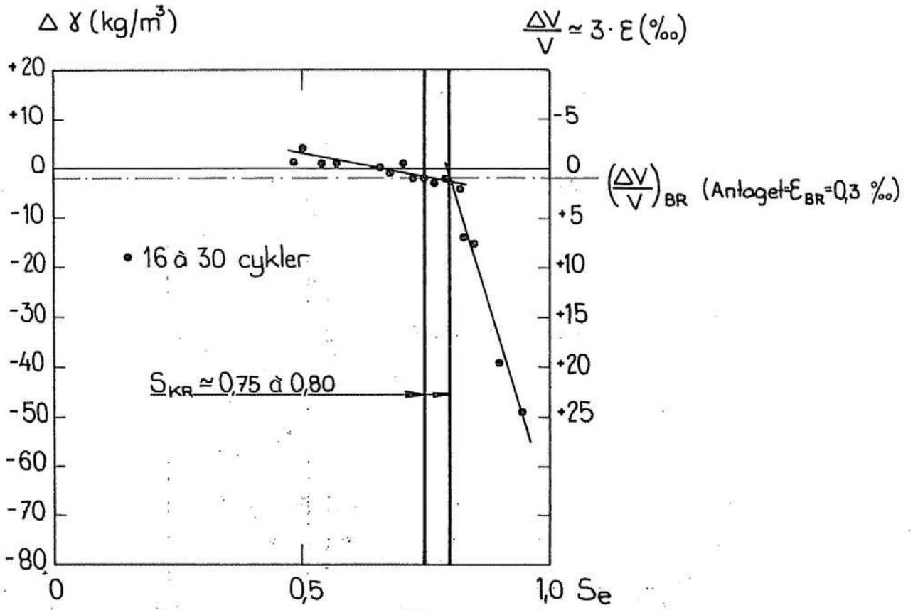
FIG 148 Material nr 14. Sarabondbruk vct=0,535. Cement mortar w/c-ratio=0,535
