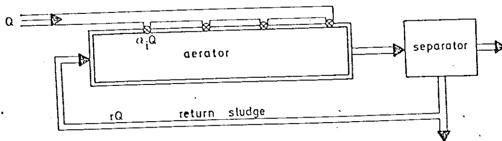
Fig. 5.2. Step loaded plug flow aerator.
