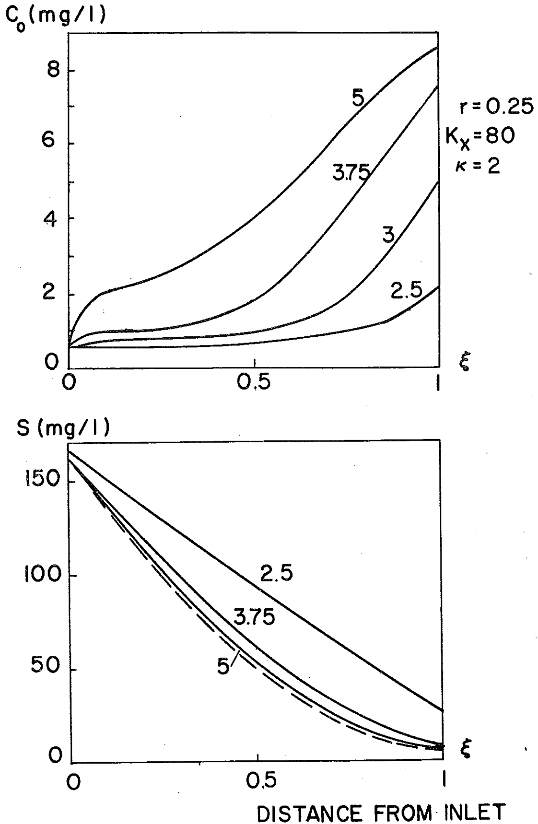
Fig. 8.3. DO and substrate concentration profiles respectively for a plug flow aerator. The value of k_{u_{air}} is the parameter. Other parameter values are given in table 8.1.
