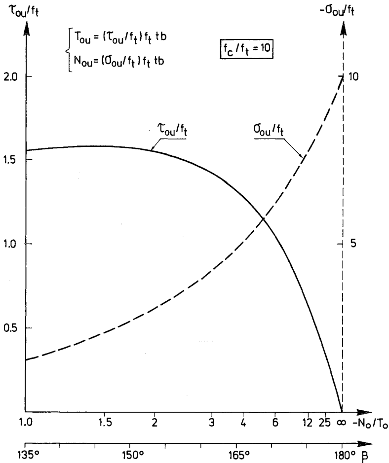
Fig 5.3 (6) a) \tau_{ou}/f_t and -\sigma_{ou}/f_t versus -N_o/T_o .
