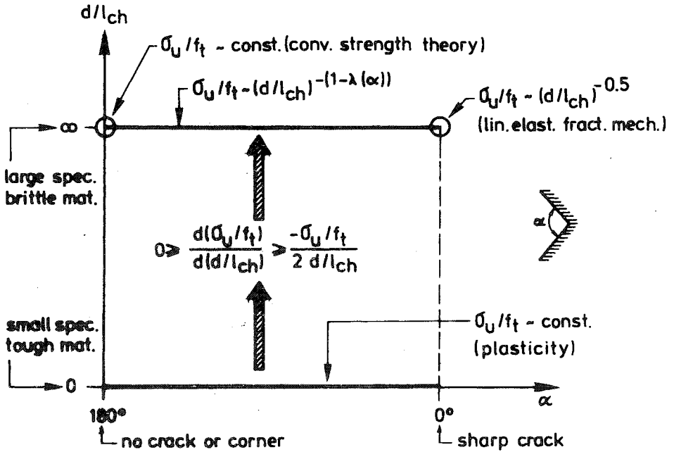
Fig 3.5 (6) Properties of the strength function \sigma_u/f_t = f(d/\ell_{ch}) at different d/\ell_{ch} and \alpha .
