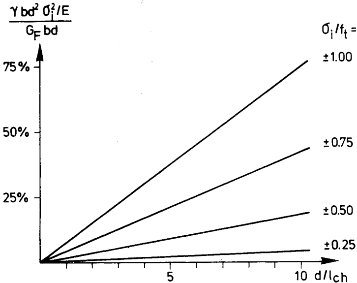
Fig 4.2 (12) Contribution from the release of strain-energy, \gamma b d \sigma_i^2 / E , to the total required work of fracture, G_F b d , vs. ratio d/l_{ch} at different magnitudes of the parabolically distributed initial internal stress.
