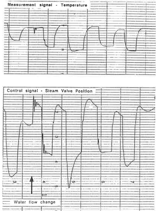
Figure 5. Adaptive control of a temperature control loop
