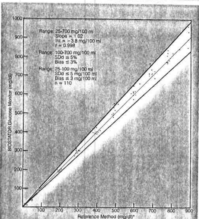
Fig. 2. Correlation curve compares the performance of the BIOSTATOR Glucose Analyzer Module with the proposed glucose reference method (hexokinase/glucose-6-phosphate dehydrogenase). 2
