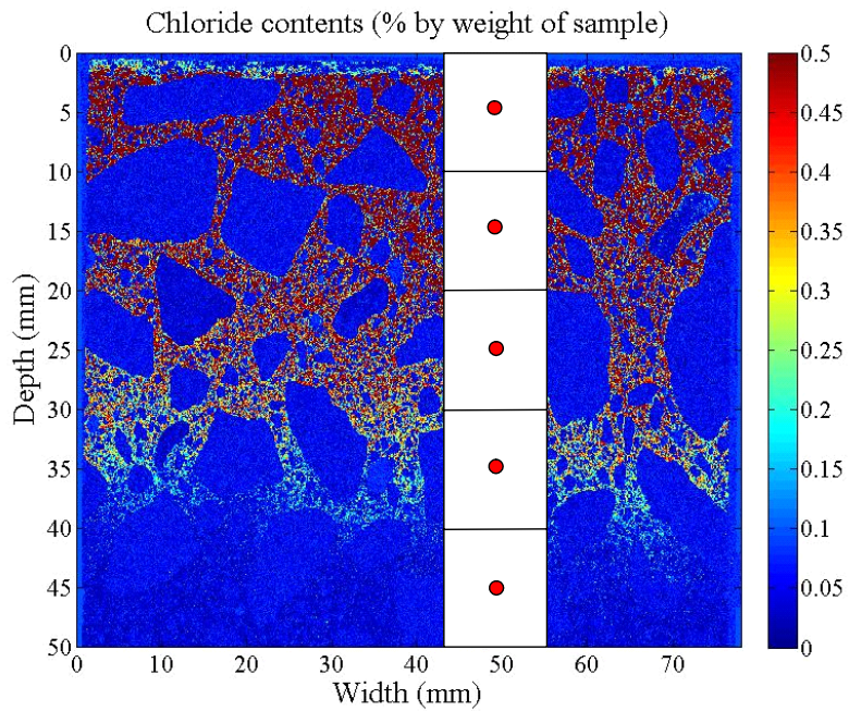
Figure 18: Chloride content in concrete specimen analyzed with EPMA showing the simulated dry drilling intervals.
