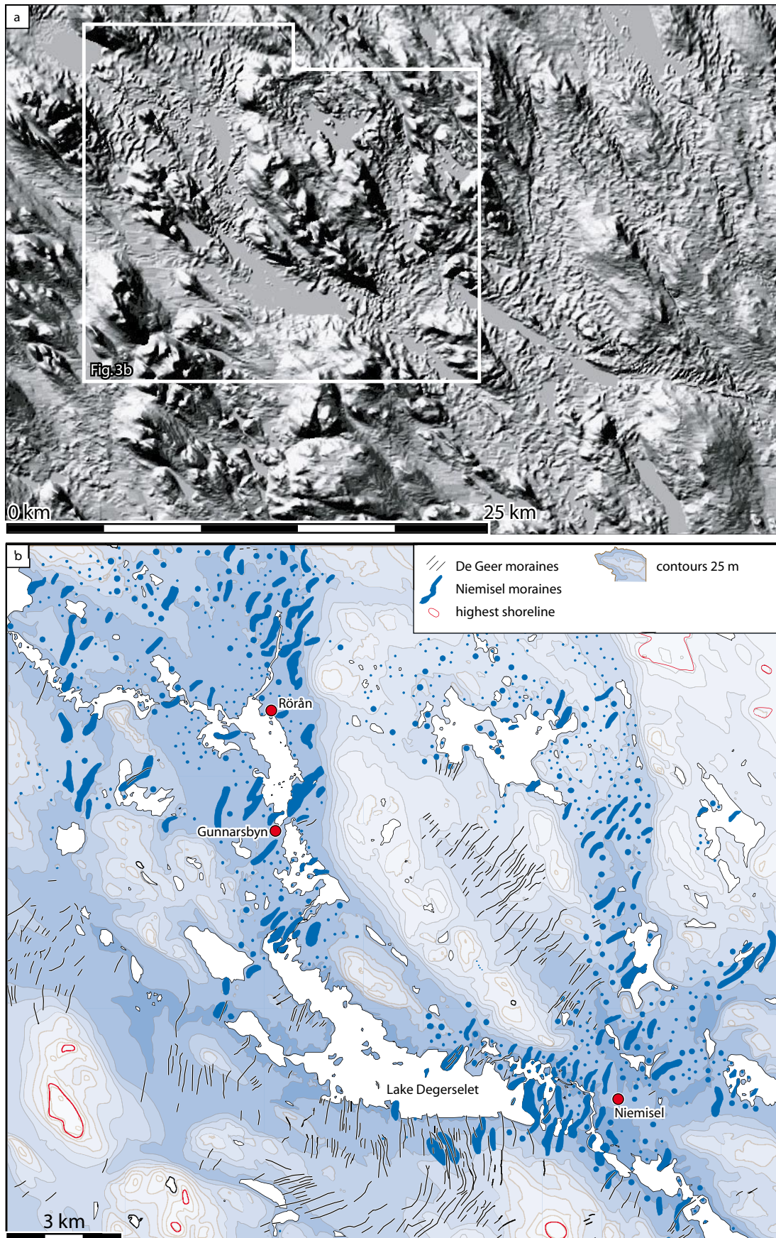
Fig. 3. (a) DEM-based relief map over the Råne River valley area. Note the dense occurrence of Niemisel moraine ridges in all low positions in the terrain, lying transverse to valley trends. Frame marks the position of Fig. 3b. (b) Detailed map over one of the investigation areas, showing the spatial distribution of De Geer and Niemisel moraine ridges. Note the occasional superimposing of De Geer moraine ridges on Niemisel moraine ridges.
