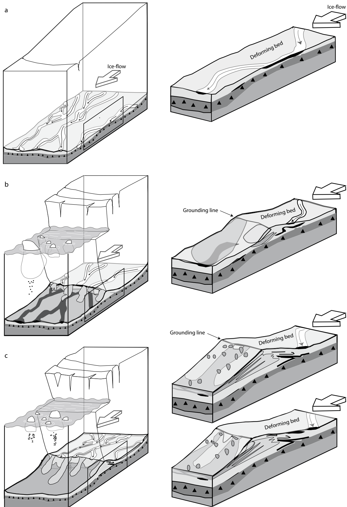
Fig. 9. Depositional model of De Geer moraine formation. Stages a-c in the figure are related to stages 1-3 in the depositional-model text, respectively, whereas stage 4 in the text correspond to the on-lapping glaciolacustrine sedimentation occurring distally of stages a-c in the figure. See text for explanation (see also Appendix II).
