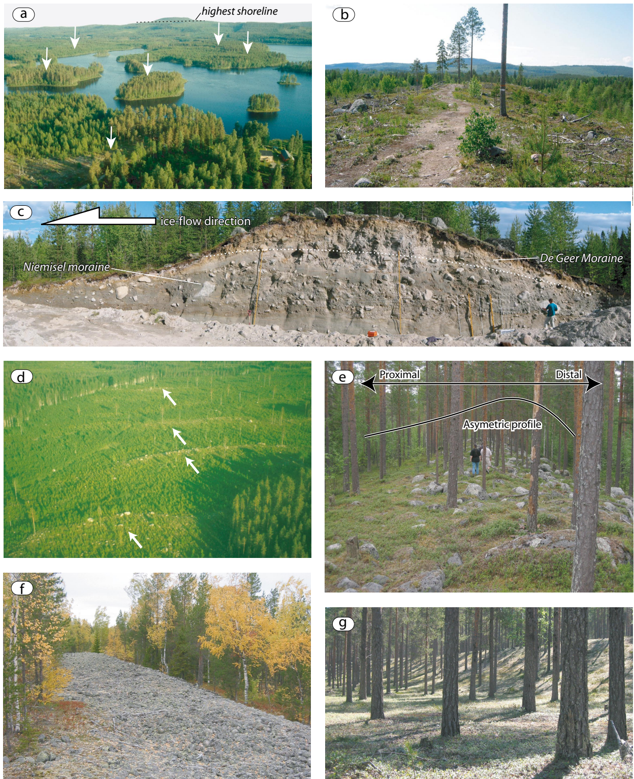
Fig. 2. (a) Morphology of Niemisel moraines at the eastern end of Lake Degerslet oblique aerial view from NNW. White arrows mark positions of individual Niemisel ridges. The height in the far background is a till-capped hill (in Swedish: kalottberg, in this case mount Snöberget demarcated with red circle at the map base, Fig. 3b), an island in the deglacial archipelago, indicated with preserved till above the highest shoreline, and with wave-washed bare bedrock and beach terraces below. (b) Longitudinal (SW) view of a Niemisel ridge. (c) Cross-sectional view at the Degerslet site, showing a De Geer moraine on top of a 90 m wide Niemisel ridge. (d) Oblique aerial photograph showing four narrow and slightly curved De Geer moraine ridges marked by arrows, also indicating the ice-flow direction. (e) Typical De Geer moraine with asymmetric cross profile and boulder concentration. Ice-flow was from left to right. (f) Cobble beach terrace close to the summit of the Sandkölen hill (c. 145 m a.s.l., Heden). (g) Sandy beach terraces (c. 70 m a.s.l.) at Heden.
