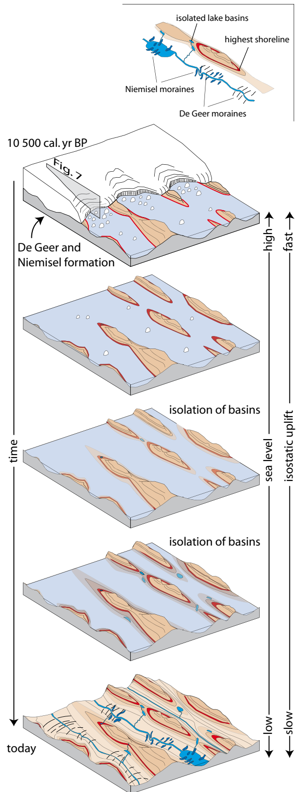
Fig. 4. Evolutionary sketch of the isostatic uplift history in Norrbotten, showing the development of the highest shoreline and the successive isolation of lake basins. The relative sea level and the isostatic uplift are further explored in Fig. 5. Frame marks the position of Fig. 7.
