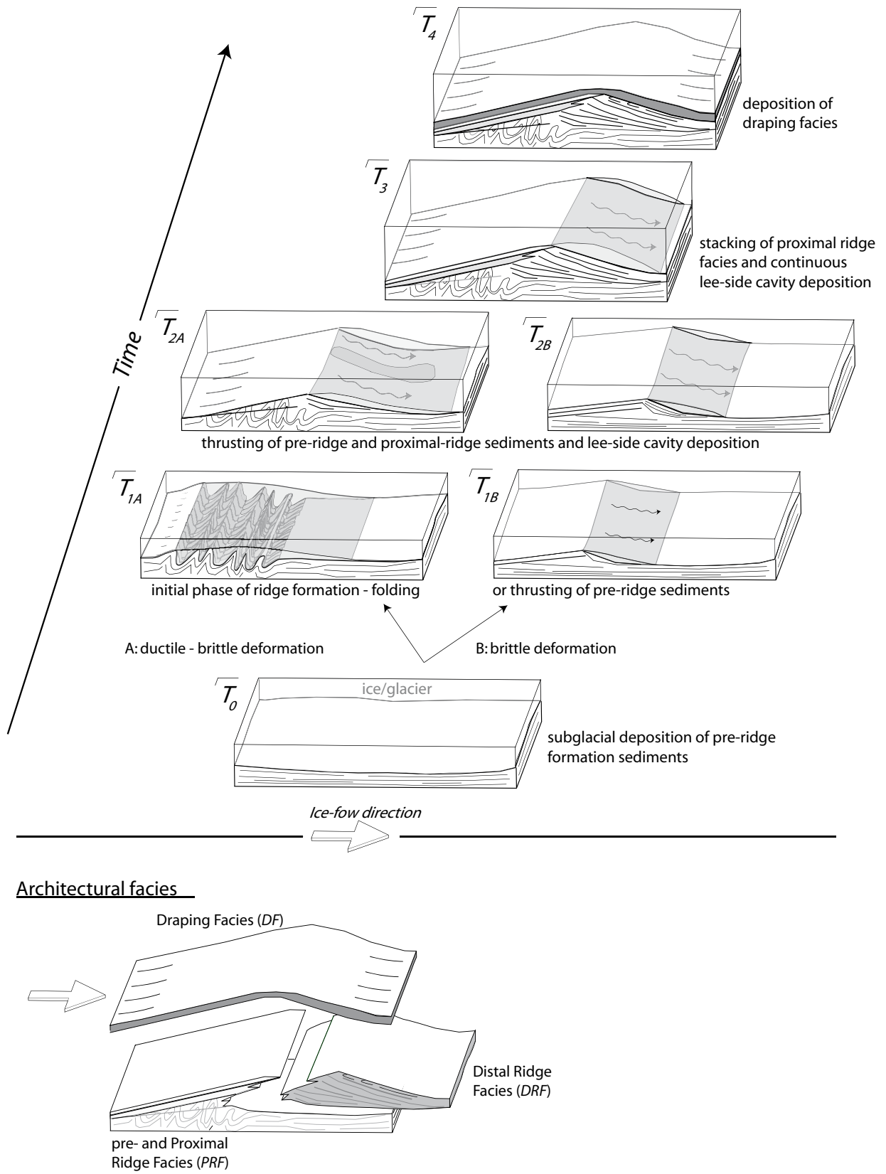
Fig. 8. Depositional model for Niemisel moraine formation. For explanations, see text (see also Appendix I).
