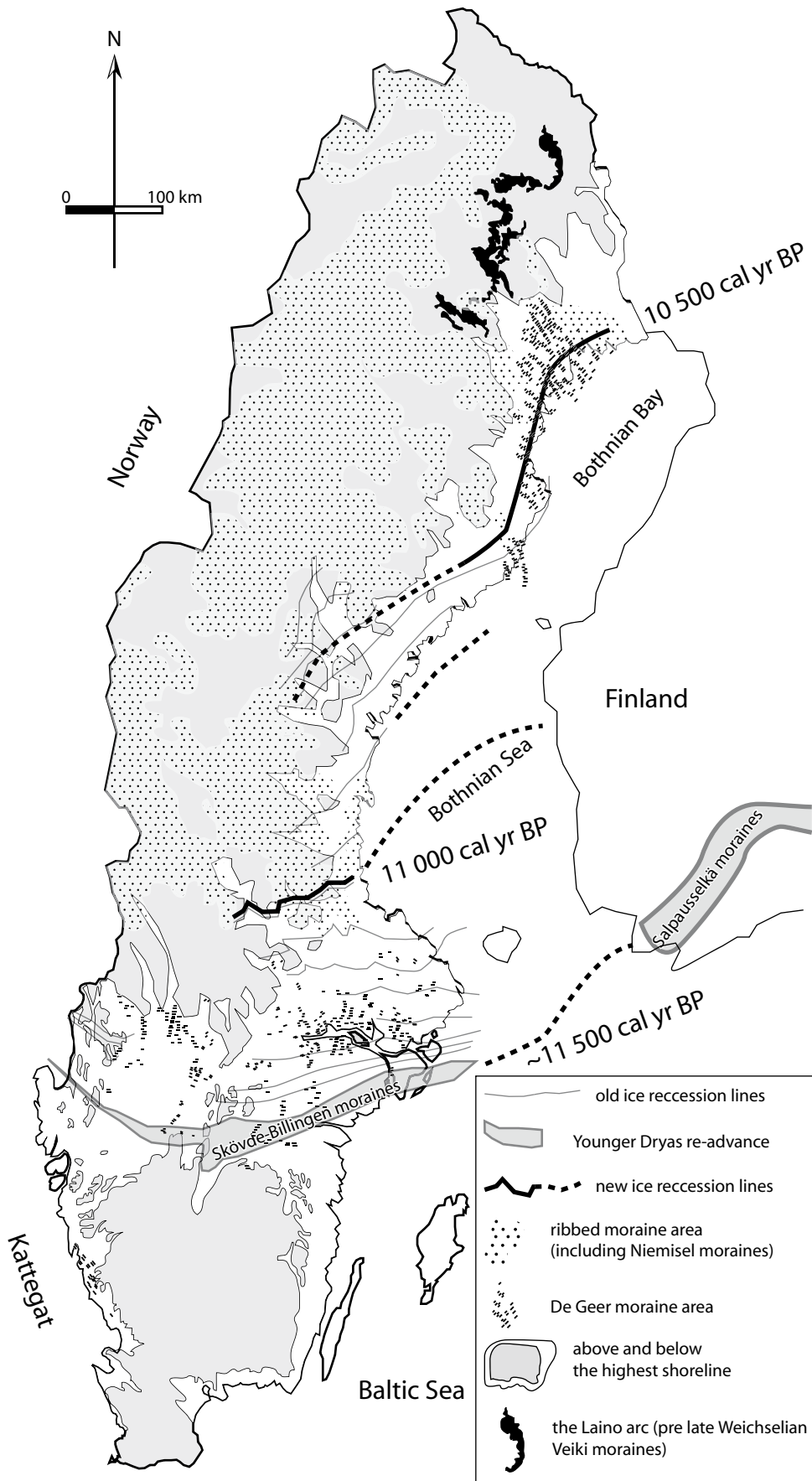
Fig. 6. Aerial distribution map of De Geer and ribbed moraines in Sweden (modified from Hättestrand, 1997b; G. Lundqvist, 1961; J. Lundqvist, 1994). Old (J. Lundqvist, 1994) and new hypothetical ice recession lines for the last deglaciation are also shown.
