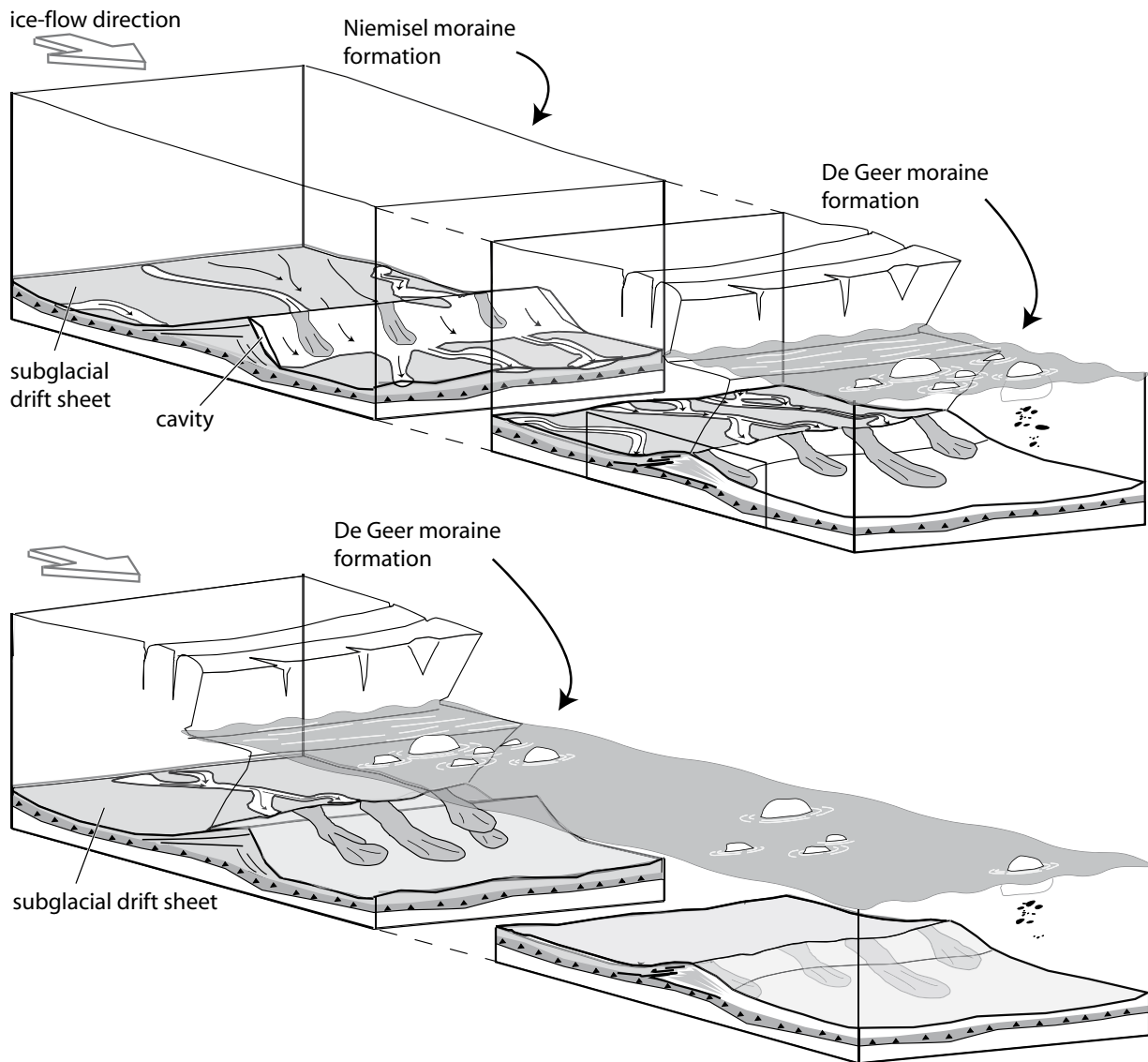
Fig. 7. Proximal-distal depositional model for Niemisel and De Geer moraine formation during subsequent recession of the ice margin.
