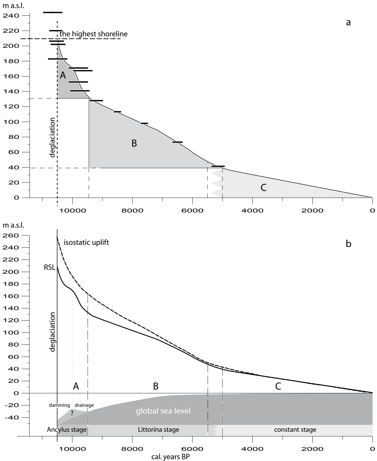
Fig. 5. (a) Relative sea level (RSL) curve for coastal Norrbotten, compiled from dated lake isolations projected to the 210 m a.s.l. highest shoreline isobase (black bars, 2\sigma age deviation or projected, see Fig. 4 in Appendix III). The different shaded areas A-C correspond to the phases in Fig. 5b: A, the Ancylus Lake stage; B, the Littorina Sea stage; C, phase of constant uplift. (b) Isostatic uplift for eastern Norrbotten (at the 210 m a.s.l. highest shoreline isobase) compiled from; - RSL + global sea level + Lake Ancylus. The global sea level curve (K. Fleming, pers. comm. 2004) is updated from Lambeck and Chappell (2001) and the Ancylus transgression (c. 10 500-9500 cal. yr BP, peaking c. 10 000 cal. yr BP) used is equivalent to a postulated 12 m up-damming of the Baltic. The isostatic uplift curve has been inverted to visualise the relationship to the RSL curve.
