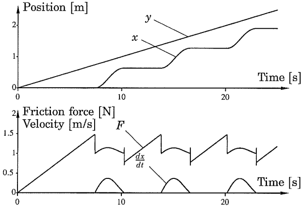
Figure 4.2 Simulation of stick-slip motion with the new model.
