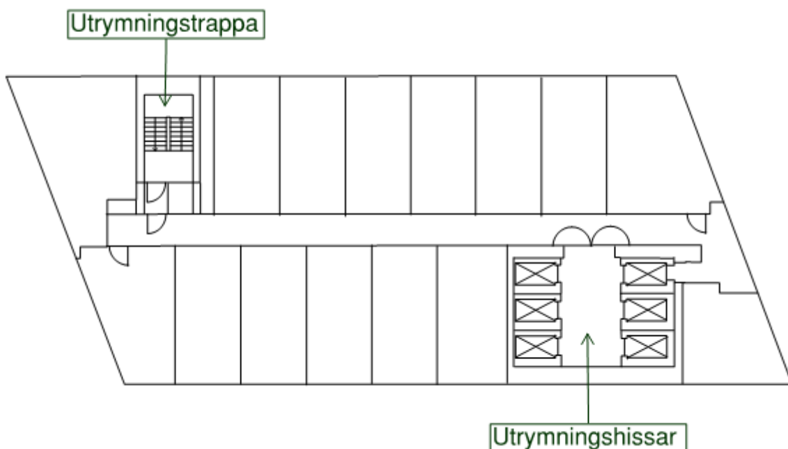
Figur 5. Hotellplanets utformning.
