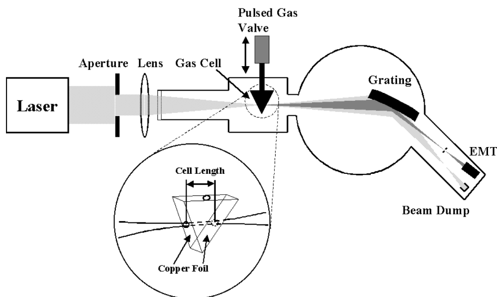
Figure 1. Experimental set-up.
