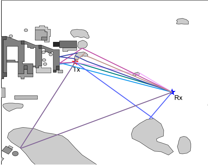
Figure 5: Visualized paths for several MPCs from one Rx position. Colors only present different MPCs.
