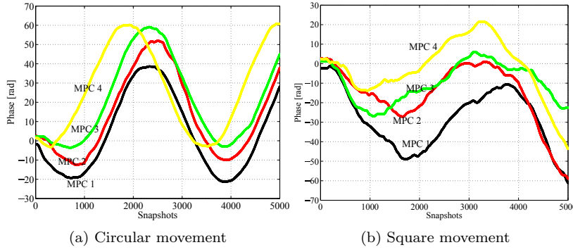
Figure 1: Tracked phases of a number of MPCs in circular and square movement measurements.
