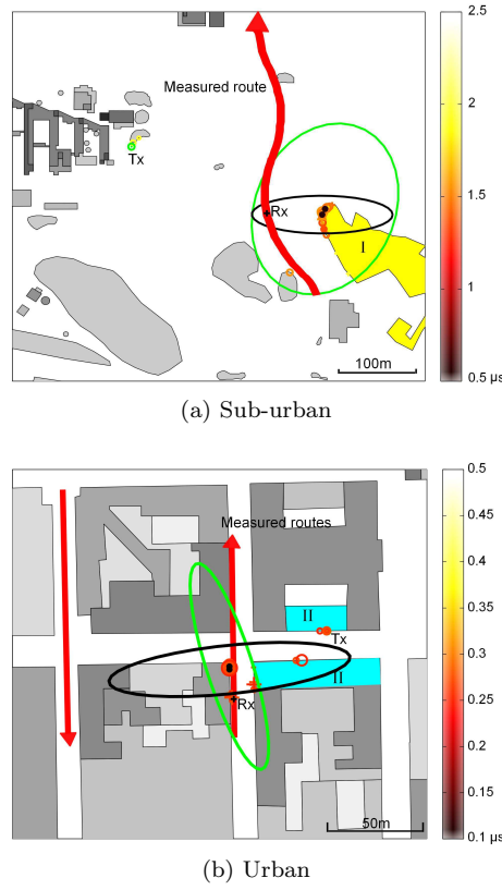
Figure 1: A visualized parameter based single-bounce cluster and the associated MPCs at a RX position in the sub-urban and urban scenarios.
