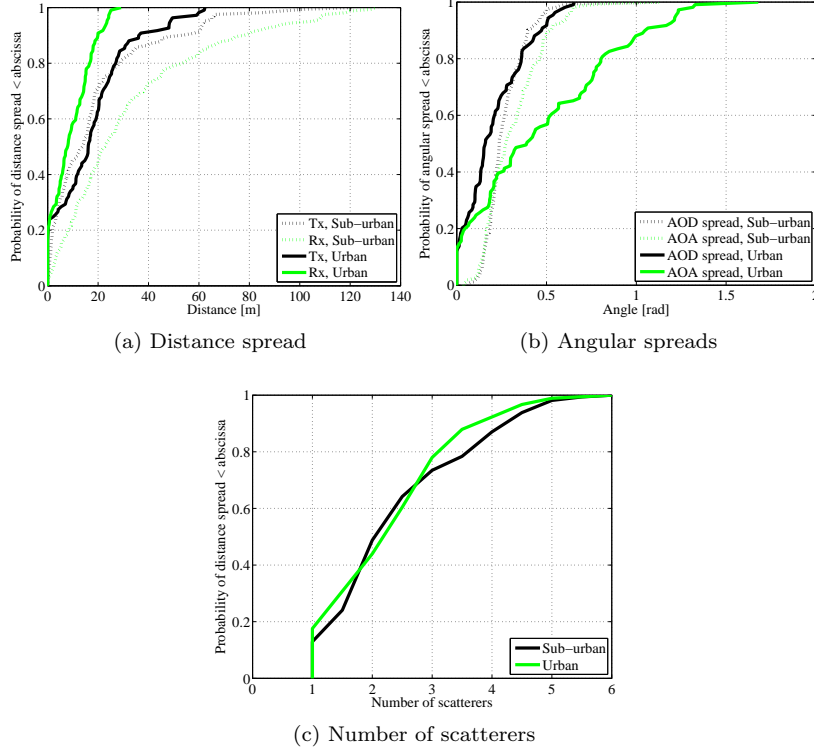
Figure 3: Properties of the interacting scatterers for the associated MPCs of a parameter based cluster: distance spread, angular spreads, number of scatterers.
