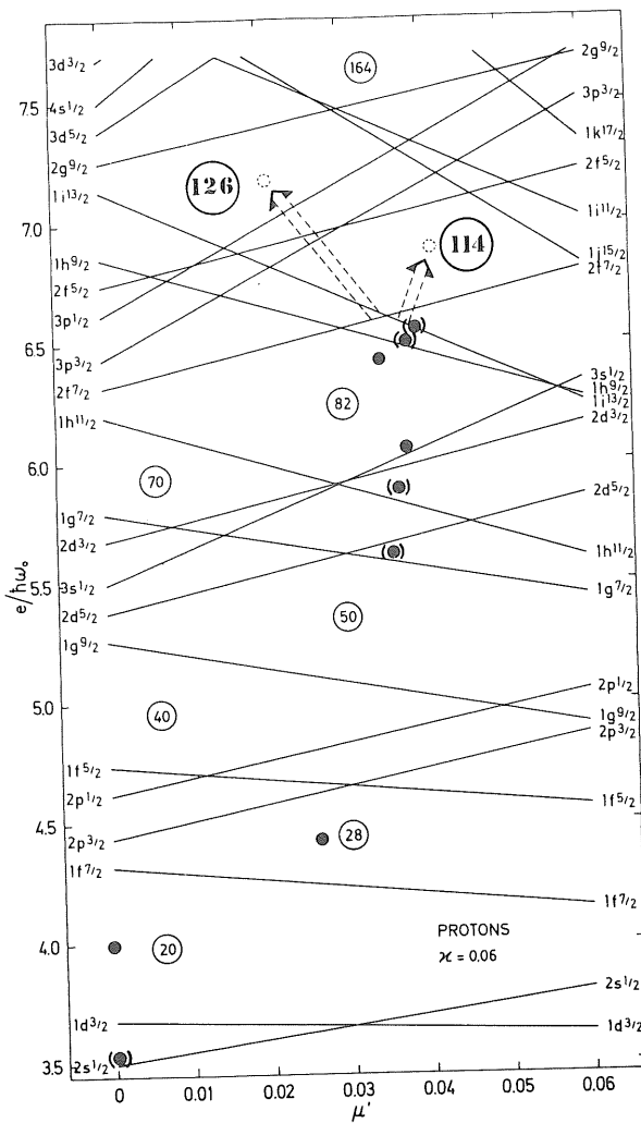
Fig. 1. Spherical single-particle levels of the M.O. potential as a function of \mu' ( = \mu\kappa ) with \kappa = 0.06 . Filled circles correspond to optimal fits to single-particle data. Circles in parentheses refer to the deformed regions. Note the extrapolation to Z = 114 and Z = 126 , the latter corresponding to an increased skin thickness of the proton potential.
