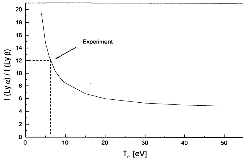
FIG. 11. Effect of initial electron temperature on Lyman- \alpha to Lyman- \beta ratio of simulated \text{He}^+ spectrum. Experimental line ratio is indicated.
