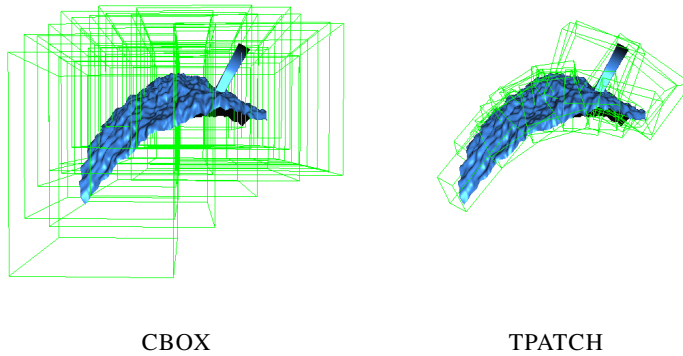
Figure 1: CBOX, which represent previous work, bounds displaced Bézier surfaces by its control points and a user-provided displacement bound. Our approach, TPATCH, uses oriented bounding boxes, a min/max hierarchy of the displacement map and an efficient normal bounding algorithm, that combined bound the patches significantly tighter.
