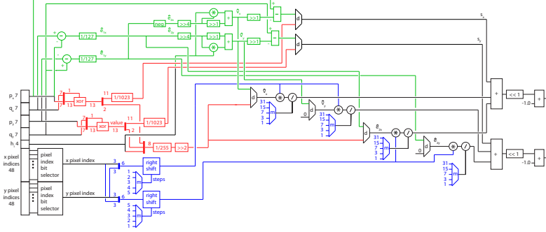
Figure 4: Diagram of a proposal for a hardware implementation of the decoder. Green: calculates \hat{\mathbf{v}} = a\hat{\mathbf{e}}_2 and \hat{\mathbf{e}}_1 which are the two vectors spanning the bounding box. It also calculates \mathbf{s} , which is the lower left point of the bounding box. Red: calculates, \hat{\mathbf{v}} , \hat{\mathbf{e}}_1 and \mathbf{s} for the differential version of the decoder. Note that, if p_x \geq q_x and p_y \geq q_y , differential data is stored in p_x, p_y, q_x and q_y . Blue: assigns the right bits for the variable bit distribution using the multiplexors marked with m . Likewise, the multiplexors marked with d choose between regular and differential input. Note that multiplication with 1/127 can be approximated efficiently as 1/128 + 1/16384 which is implementable with shifts and additions (not shown). Likewise for 1/255 and 1/1023 .
