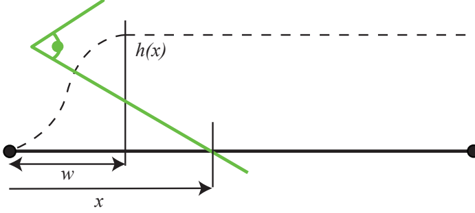
Figure 8: A frustum plane (green) is intersecting a triangle edge (bold black). Based on the parametric coordinate x \in [0, 1] along the edge, we apply a smooth step-function h(x) \in [0, 1] , so that in the transition zone, x \in [0, w] , h(x) specify a smooth blending weight. Thus, as the triangle edge intersect the frustum plane, the edge will transform smoothly from non-uniform to regular fractional tessellation.
