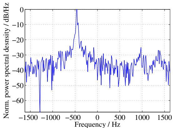
Figure 10: Doppler profile at delay-tap k = 33 (138 ns)
