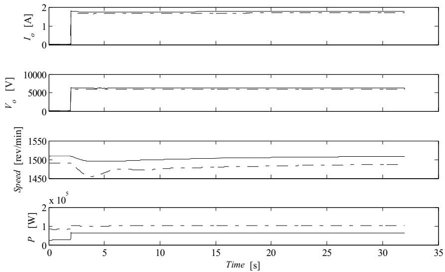
Figure A1.1.6 Phase A to earth fault. Zero sequence current and voltage at fault point, generator speed, generator active power. P_{load} = 5 \text{ kW} (solid lines) and P_{load} = 85 \text{ kW} (dashed lines). L_{L1} = 4 \text{ km} , R_f = 0 \Omega
