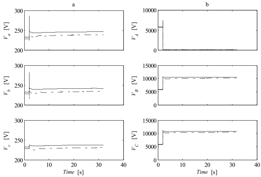
Figure A1.1.5 Phase A to earth fault. a) Phase voltages at induction generator terminals b) Phase voltages on the high voltage side of step up transformer. P_{load} = 5 \text{ kW} (solid lines) and P_{load} = 85 \text{ kW} (dashed lines). L_{L1} = 4 \text{ km} , R_f = 0 \Omega
