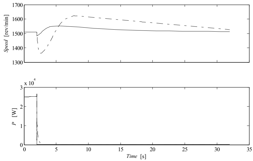
Figure A1.9.9 Three Phase fault. Generator speed, generator active power. l_{L1} = 2 \text{ km} (solid lines) and l_{L1} = 6 \text{ km} (dashed lines). Pload = 5 kW, R_f = 0 \Omega
