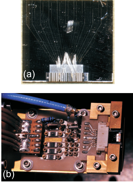
FIG. 9. Cold finger inside the 10 K closed-cycle refrigerator: (a) Image of the TiAu metal-metal waveguide laser bar, 1049 \mu\text{m} long, soldered onto a high-resistive Si carrier. The fan-out electrodes deposited on carrier can be seen, but with a low contrast due to their small thickness; this is why they showed a residual resistivity. (b) The laser bar mounted on the cold finger. The blue wire is a 18-GHz SMA cable used for voltage detection and on the other side, it is connected to a 50- \Omega input channel of a high-bandwidth oscilloscope. About 25 mm separate the laser bar from the SMA cable with, in between, a circuitry that is not optimized for RF.
