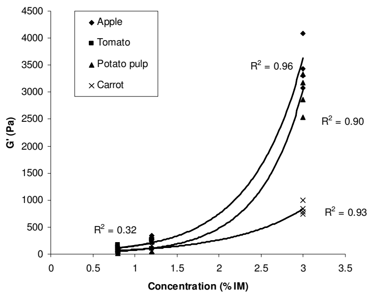
Figure 17. The effect of concentration on the elastic modulus of dietary fibre from different sources.
