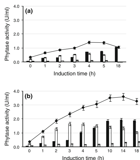
Fig. 1 Distribution of the expressed recombinant phytase in shake flask cultivation of E. coli BL21(DE3) at 30°C. Cells grown a without \text{CaCl}_2 and b with 10 mM \text{CaCl}_2 during enzyme induction. Symbols: Total phytase activity (filled diamond), and activity in cell free fraction (filled bar), periplasmic fraction (open bar) and cytoplasmic fraction (gray bar)
