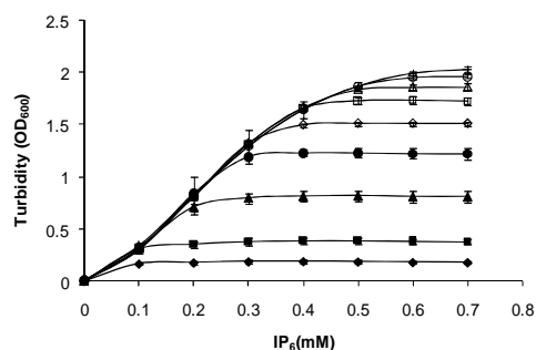
Fig. 1. Effect of IP_6 and lysozyme concentration on the turbidity of IP_6 -lysozyme complex solution. The complex was prepared in 50 mM sodium acetate buffer pH 4 containing 0-0.7 mM IP_6 and lysozyme at different concentrations: 30 \mu M (♦), 58 \mu M (■), 116 \mu M (▲), 174 \mu M (●), 231 \mu M (◊), 289 \mu M (□), 347 \mu M (Δ), 405 \mu M (○), and 463 \mu M (+) in a total volume of 120 \mu l. Experimental details are described in the Materials and Methods section.
