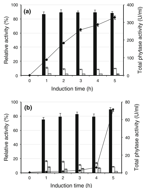
Fig. 5 Distribution of recombinant phytase with time during fed-batch cultivation in 2.5 l culture medium induced by a 1 mM IPTG and b 20 mM lactose: relative activity in extracellular (filled bar), periplasmic and (open bar) cytoplasmic (gray bar) fractions, and total phytase activity (filled diamond)
