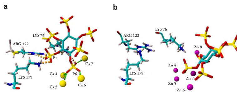
Fig. 7 a) Top view of \text{IP}_6 docked into calcium loaded phytase; dashed lines are hydrogen bonds; green arrows indicate the interaction of the 4 \text{Ca}^{2+} ions (Ca4-Ca7) and the phosphate group (P6) at the cleavage site, b) Side view of effect of zinc binding to phytase: \text{IP}_6 is disoriented in the cleavage site and the phosphate group (P6) lies outside the four Zn atoms. Adaptation of Lys 179 side chain to form hydrogen bond is noticed in case of Ca-phytase. The molecular graphics were created with YASARA ( www.yasara.org ) and PovRay ( www.PovRay.org ).
