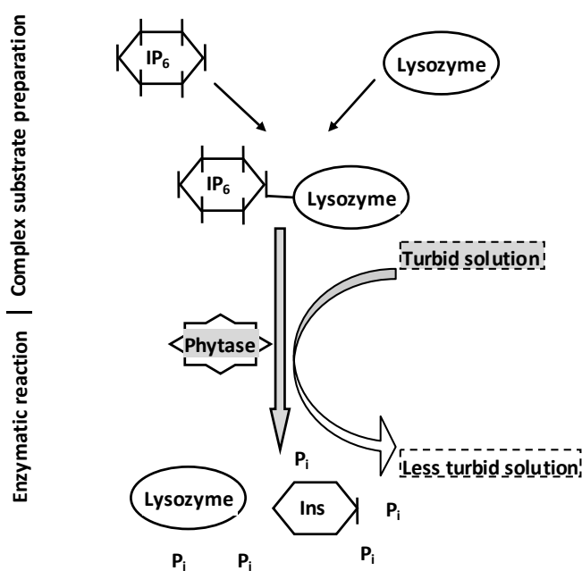
Figure 2.4 Scheme of the kinetic assay of phytase activity.
