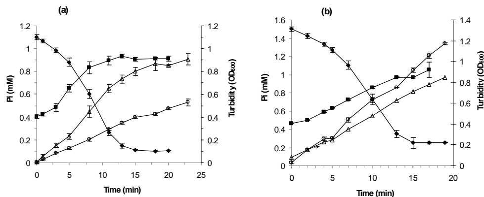
Fig. 5. Activity of (a) E. coli phytase variant 1 (0.1 FTU/ml) and (b) A. niger phytase (0.5 FTU/ml) with IP_6 -lysozyme substrate based on turbidity reduction (◆) and P_i released (■); with IP_6 based on P_i released (△); and with IP_6 -lysine complex based on P_i released (○). The three substrates were prepared in 50 mM glycine-HCl (pH 3.5) containing 0.3 mM IP_6 (for IP_6 substrate) and either lysozyme 0.23 mM (for IP_6 -lysozyme substrate) or lysine 23 mM (for IP_6 -lysine substrate) in a total volume of 120 \mu l. Reactions were performed at 37°C for 25 min with continuous mixing. Turbidity of the reactions was determined every 30 sec. For P_i determination, the reactions were stopped by adding 30 \mu l of 2.5 M HCl, centrifuged and the supernatants were analyzed for P_i on Konelab.
