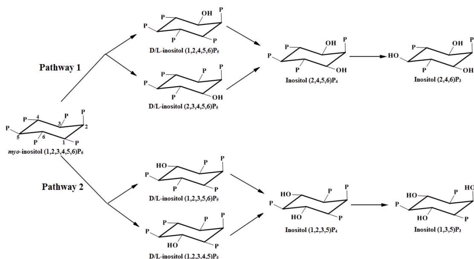
Figure 3.5 Scheme of the \text{IP}_6 hydrolysis pathways of Phytase C from Bacillus subtilis VTTE 68013 (redrawn according to Kerovuo et al., [232]). P stands for \text{H}_2\text{PO}_4^- .
