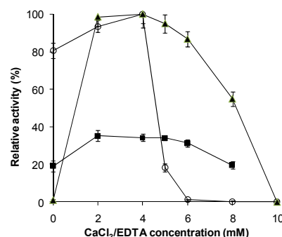
Fig. 5 Effect of \text{CaCl}_2 and EDTA concentration on the activity of recombinant Bacillus sp. MD2 phytase. The assays were performed at pH 7, 37 °C ( \blacksquare ) and at 70 °C ( \blacktriangle ) with different concentration of \text{CaCl}_2 . The effect of EDTA ( \circ ) concentration was investigated at 70 °C.
