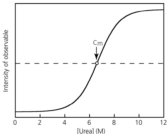
Figure 4. Hypothetical 2-state urea denaturation where \Delta G^{\circ}_{\text{DN}}(\text{H}_2\text{O})=19.4 kJ/mol, m=2.9 kJ/(mol·M) and T=298.15 K.
