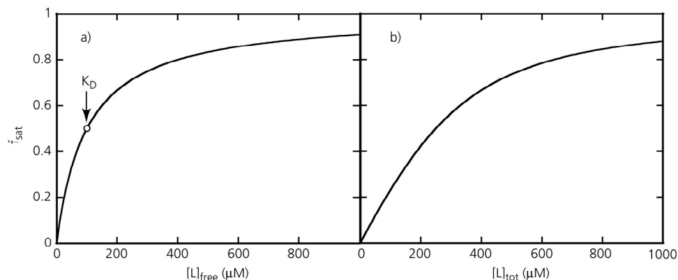
Figure 8. Hypothetical ligand binding obtained by using Equation 35 (a) and 36 (b) with K_D=100\text{ }\mu\text{M} and [P]_{\text{tot}}=300\text{ }\mu\text{M} .
