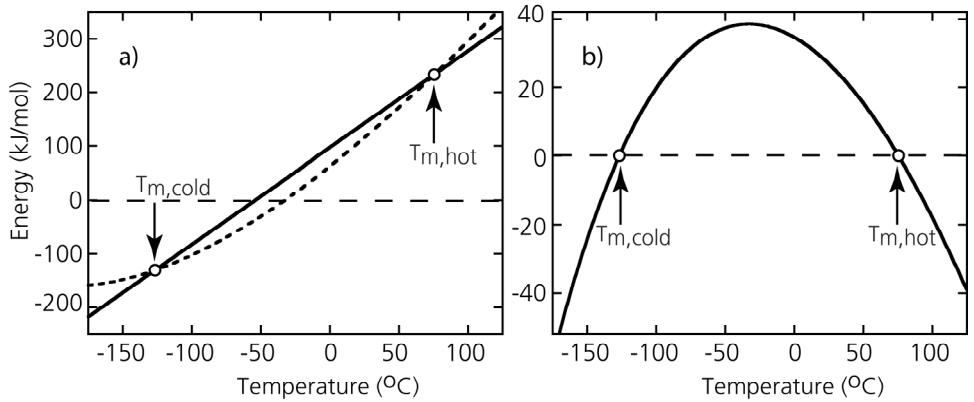
Figure 2. Temperature dependence of a) \Delta H^\circ_{\text{DN}} (solid line), T\Delta S^\circ_{\text{DN}} (dashed line) and b) \Delta G^\circ_{\text{DN}} for PGB1-QDD at pH 5. The figure is generated using values determined in paper I ( \Delta H^\circ_{\text{DN}} = 233 kJ/mol, \Delta C^\circ_{\text{p,DN}} = 1.8 kJ/(mol·K), T_m = 75.5^\circ\text{C} ). The cold and heat denaturation points are indicated but for this protein the cold denaturation occurs at an extremely low temperature and is just a hypothetical point. Note the different scales of the y-axis in a and b and that the curve in b arises from the small difference between the curves in a.
