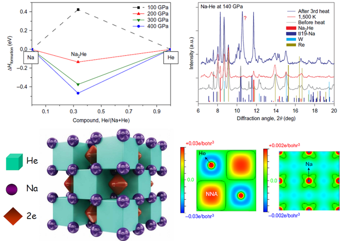
Figure 12. \text{Na}_2\text{He} : ( Top left ): predicted convex hulls of the Na-He system, based on the theoretical ground states of Na and He at each pressure. The calculated \Delta H_{\text{formation}}(\text{Na}_x\text{He}_{1-x}) = xH(\text{Na}) + (1-x)H(\text{He}) - H(\text{Na}_x\text{He}_{1-x}) ( H = enthalpy) indicates that \text{Na}_2\text{He} has a lower enthalpy, hence is thermodynamically more stable, than the mixture of elemental Na and He, or any other mixture, at pressures above 160 GPa. ( Top right ): Synchrotron XRD data. Below 113 GPa only single crystal reflections of elemental Na were observed, whereas above this pressure new single crystal reflections appeared, which became even stronger after laser heating to a temperature > 1500 K. Vertical ticks correspond to expected positions and intensities of XRD peaks of \text{Na}_2\text{He} , tI19-Na, Re (gasket) and W (pressure gauge). ( Bottom left ): Geometric and electronic structure of \text{Na}_2\text{He} . ( Bottom right ): Interaction density in the (100) plane of \text{Na}_2\text{He} passing through He atoms. This quantity was obtained by making separate calculations on the Na and He sublattices (i.e. \text{Na}_2\text{He} without He and without Na, respectively) and subtracting the resulting electron densities from that of \text{Na}_2\text{He} . NNAs indicate interstitial electron localizations. Insertion of He pushes electron density out, causing its interstitial localization. Adjusted from Figures 1, 3 and 4 with permission from reference [256] and (bottom right) from Figure 1 in reference [265] , with permission from and credit to Artem Oganov, Skolkovo Institute, Moscow, Russia.
