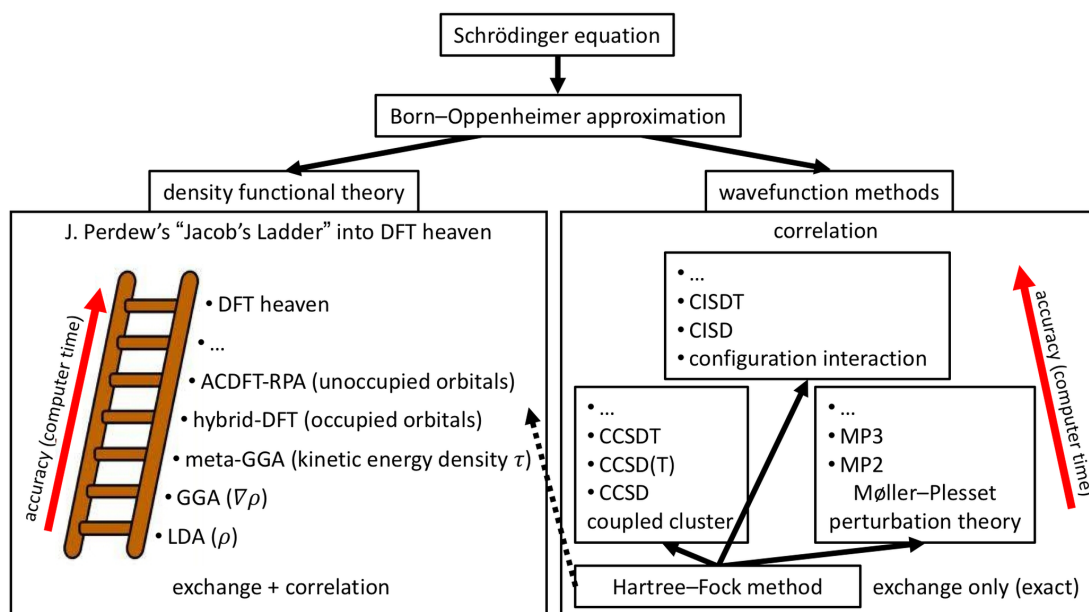
Figure 2. The most important quantum mechanical approximations and methods. The many-particle Schrödinger equation is simplified using the Born–Oppenheimer approximation. From there, one route is DFT and the other is the HF method. The most important post-HF methods that approximate electron correlation missing in HF are based on Coupled Cluster (CC) and Configuration Interaction (CI) techniques as well as the Møller–Plesset (MP) perturbation theory.
