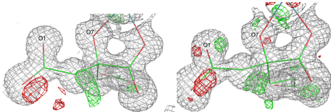
Figure 4. Electron-density maps of two possible protonation states of the homocitrate ligand in nitrogenase. [149] The 2mF_o - DF_c maps are contoured at 1.0 \sigma and the mF_o - DF_c maps are contoured at +3.0 \sigma (green) and -3.0 \sigma (red). The structure to the left fits the experimental data better, especially around the O1 and O7 atoms. This is also reflected by the real-space difference density Z-scores, which are 3.0 and 3.2, respectively. Reprinted with permission from reference [149] (Copyright 2017 American Chemical Society).
