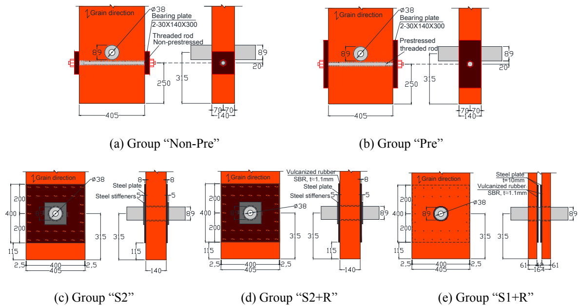
Figure 1: Configuration of test specimens. Units: [mm]
