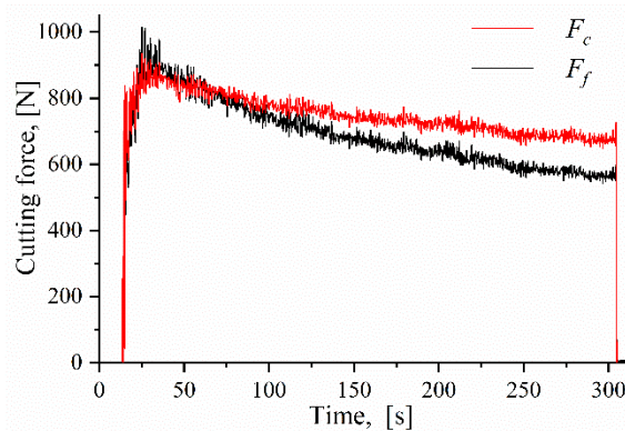
Fig. 11. Cutting F_c and feed F_f force components for the CC1 machining test.
