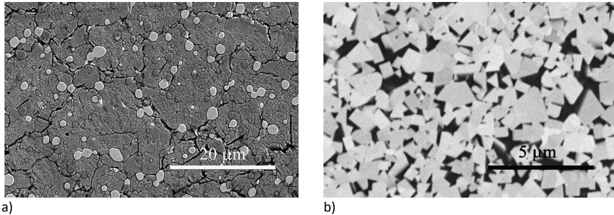
Fig. 4. Microstructures of tools.
