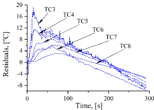
Fig. 30. Signed residuals between measured temperatures and calculated for assumed constant heat flux: a) HSS1, b) HSS2, c) CC1, and d) CC2.
