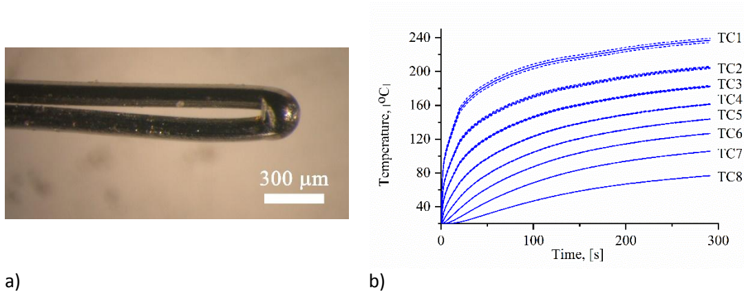
Fig. 18. (a) Optical micrograph of actual thermocouple junction, and (b) influence of its size on the modeled temperature in control points.
