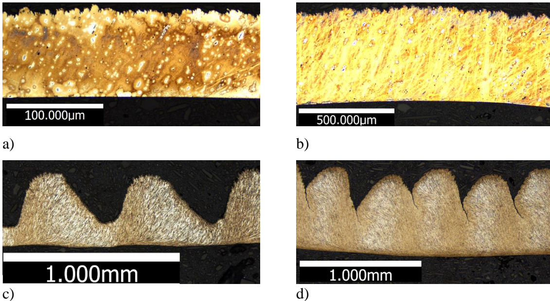
a) b) c) d) Fig. 15. Optical micrographs of the chip cross section for (a) HSS1, (b) HSS2, (c) CC1, and (d) CC2 cutting tests
