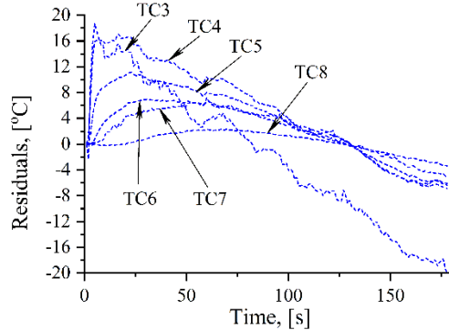
Fig. 30. Signed residuals between measured temperatures and calculated for assumed constant heat flux: a) HSS1, b) HSS2, c) CC1, and d) CC2.
