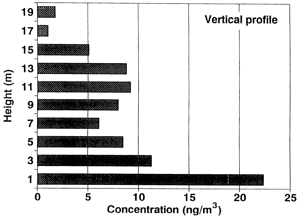
Figure 5. Vertical profile of Hg over a roasted cinnaber deposit.
