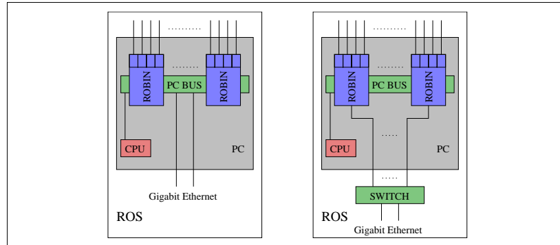
Figure 5-5 Bus and switched based ROS
