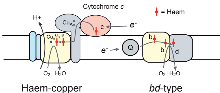
Figure 4 | Pictures of a haem-copper enzyme compared to a bd -type. The haem-copper enzyme has a binuclear centre containing \text{Cu}_B and a haem molecule while the bd -type enzyme probably uses two haem cofactors at the active site.
