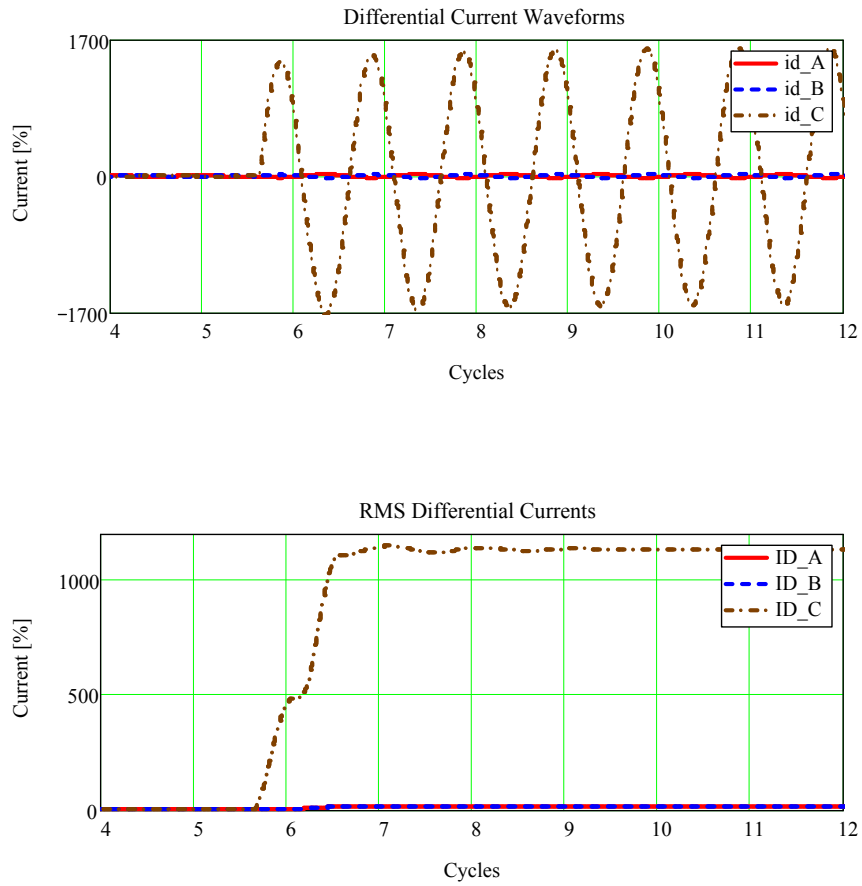
Figure 67: Differential currents during this internal fault
