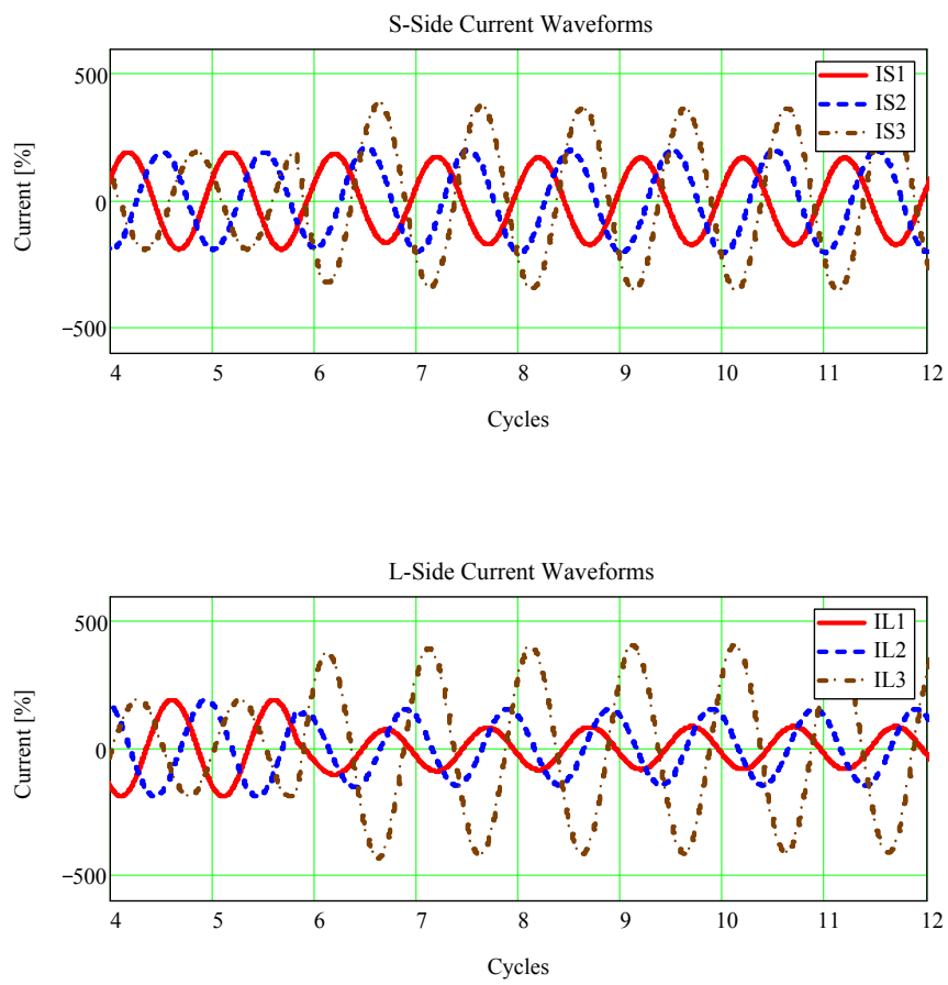
Figure 56: Individual phase currents during this external fault
