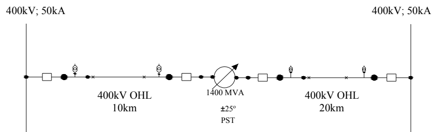
Figure 47: SLD for the simulated power system.
