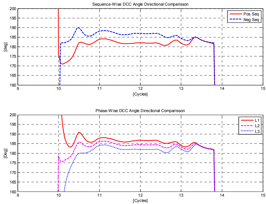
Figure 98: Directional comparison during internal fault.
