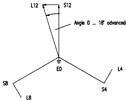
Figure 29: Part of rating plate for dual-core, asymmetric PST design.
