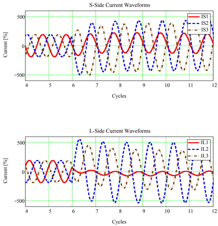
Figure 54: Individual phase currents during this external fault
