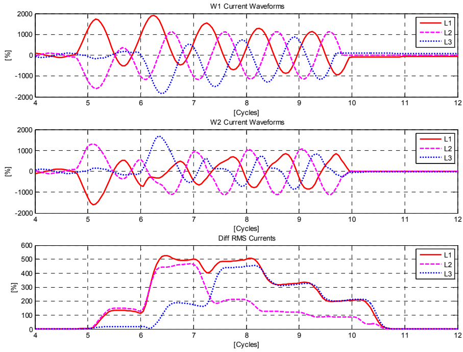
Figure 95: External L1-L2 fault evolving into a three-phase fault on the 35kV side.
