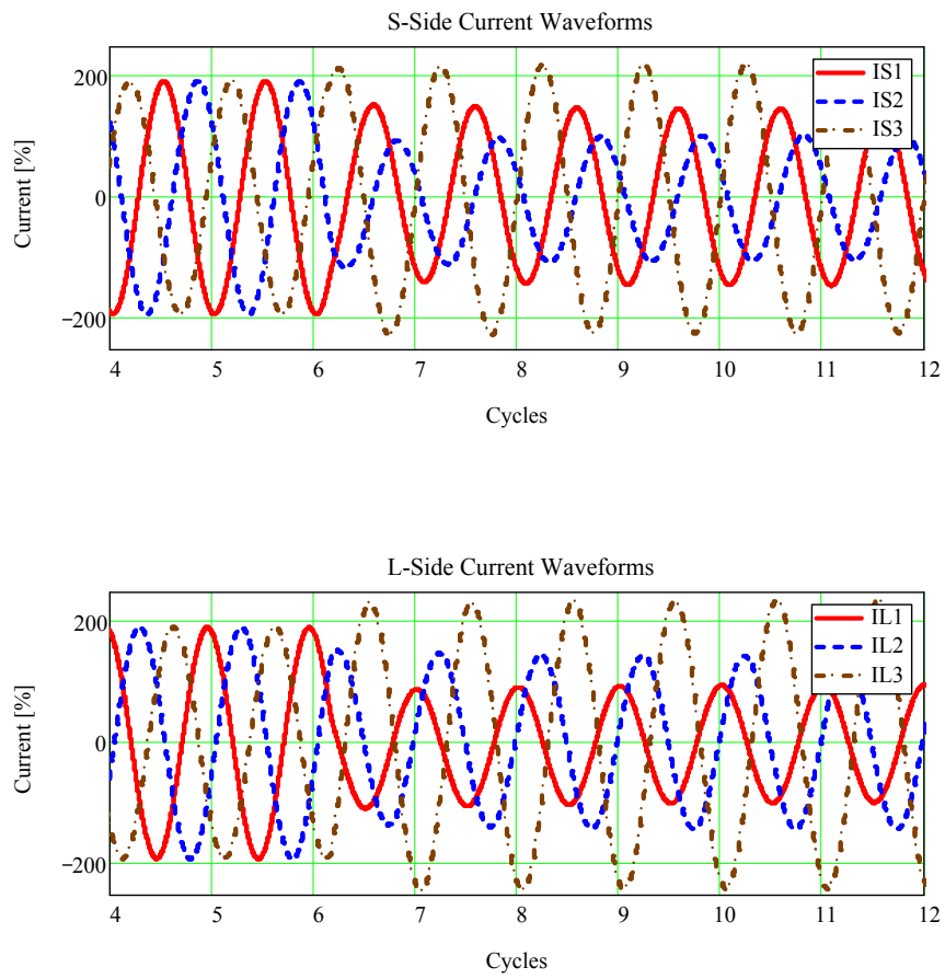
Figure 62: Individual phase currents during this internal fault
