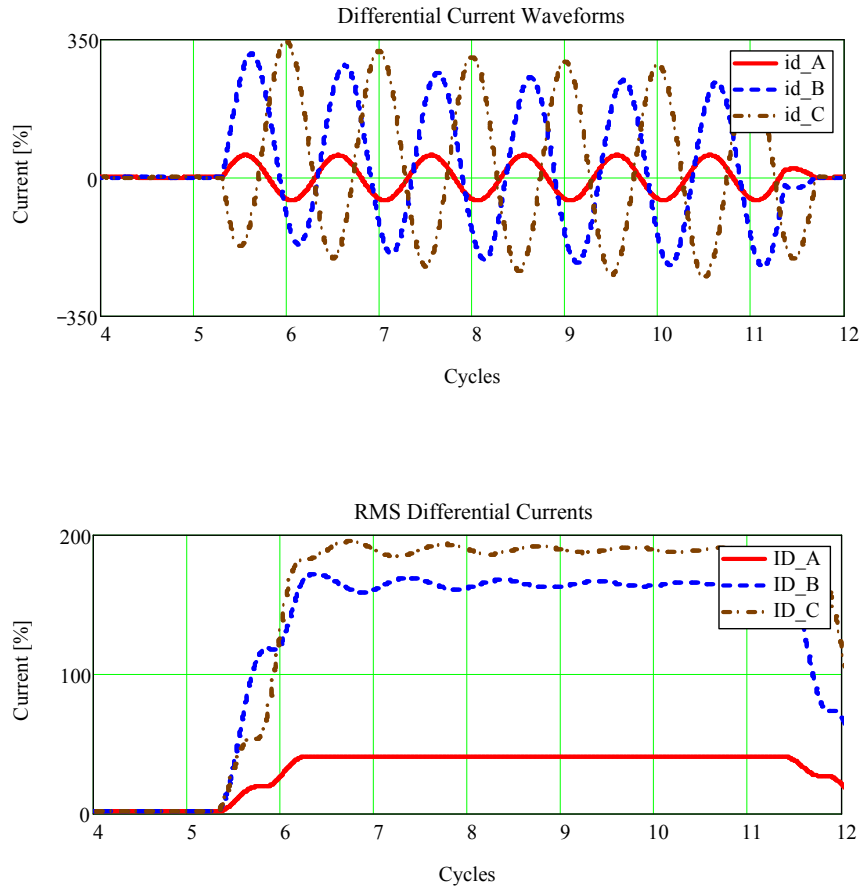
Figure 61: Differential currents during this internal fault
