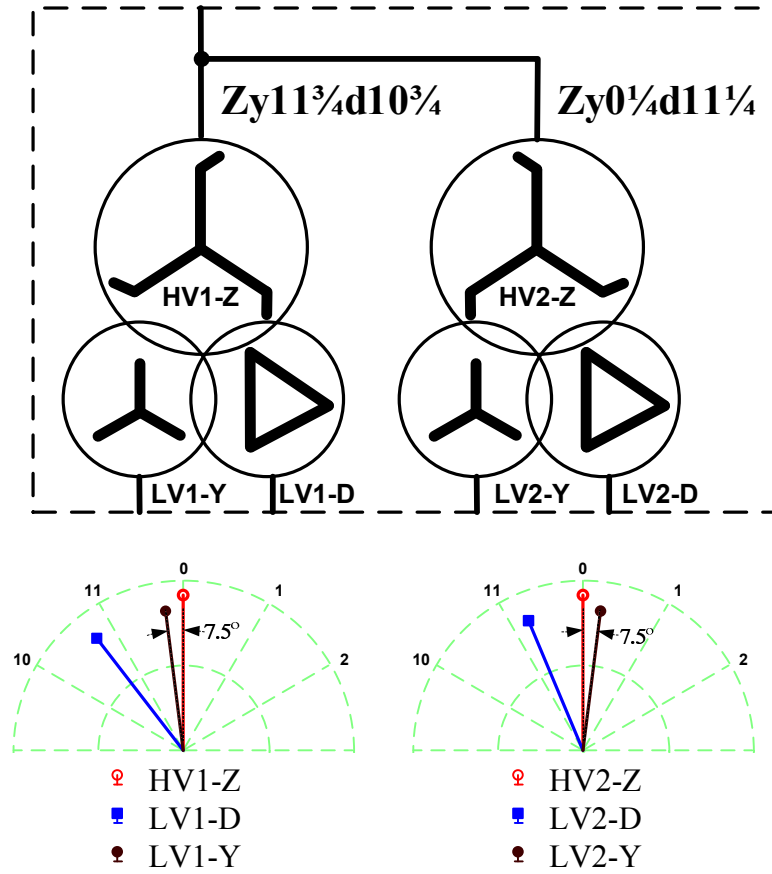
Figure 73: 24-pulse converter transformer with positive sequence phasor diagram.
