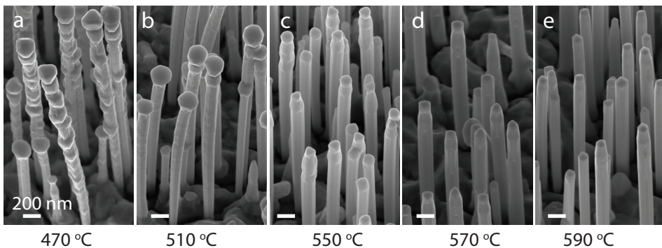
Figure 5.13 30° tilted SEM images of \text{GaAs-GaAs}_x\text{Sb}_{1-x} core-shell nanowires where the \text{GaAs}_x\text{Sb}_{1-x} shells were grown at (a) 470 °C, (b) 510 °C, (c) 550 °C, (d) 570 °C, and (e) 590 °C with an Sb flux of 1.6 \times 10^{-6} Torr. The temperature of the Ga effusion cell was fixed to obtain a nominal planar GaAs growth rate of 0.7 \text{ ML s}^{-1} on a GaAs (100) substrate, together with an As flux with a beam equivalent pressure of 5.6 \times 10^{-6} Torr. The scale bars for (b-e) are 200 nm. Part of the figure has been adapted from Paper V.
