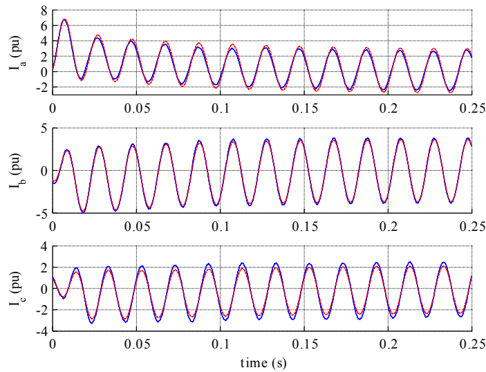
Figure 3.10 Simulated (solid blue) and calculated (dotted red) high voltage side short-circuit current for a phase-ground ( a-g ), with parameter p=0.99 . Pre-fault voltage angle \varphi=90^\circ . Initial apparent power S=0.8-j0.25 pu, rotor speed \omega_r=1.25 pu. The voltage on the high voltage side is 130 kV and a zig-zag transformer is used to create a direct grounding.
