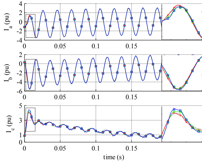
Figure 3.6 Simulated with instantaneous (red +), 2.5 ms delayed (green \diamond ), 5 ms delayed (blue \square ) crowbar insertion and calculated (black dotted) DFIG short-circuit current for a phase-phase ( b - c ) fault, with parameter p=0.8 . Pre-fault voltage angle \varphi = 0^\circ . Initial apparent power S=0.8-j0.25 pu, rotor speed \omega_r=1.25 pu.
