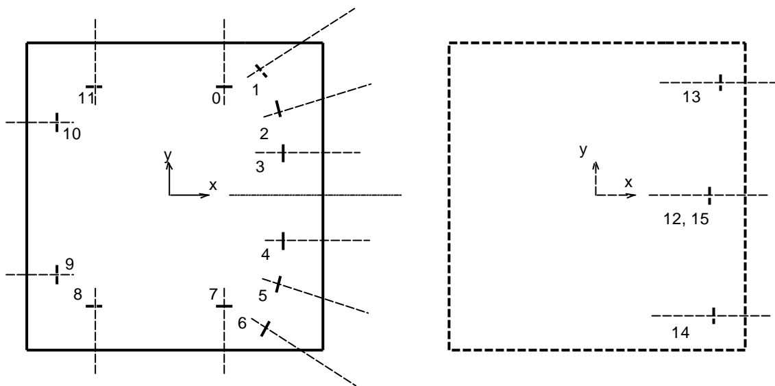
Figure 7. The extended sensor configuration.
