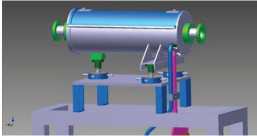
Figure 3: Quadrupole lens with ceramic tub and supply conductors mounted on the frame.(Picture: GSI).
