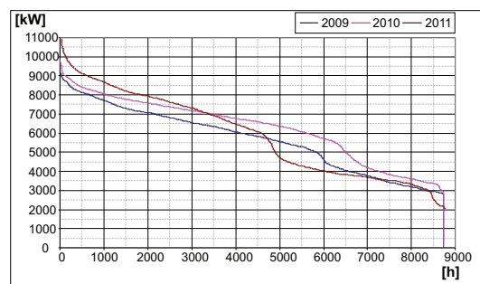
Figure 2: Distribution of power loads in a 15 minute average caused by GSI campus and accelerator facility. Note the difference in load from 5000 h to 6500 h due to different operation times of the accelerator (taken from [5]).
