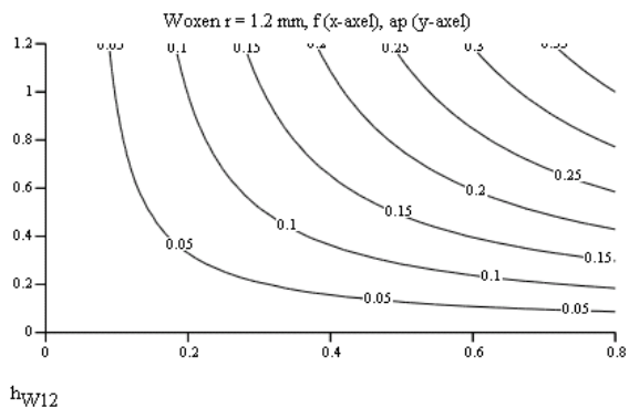
Figure 11. Deviations in % between true chip equivalent h_e and Woxén's chip equivalent h_{eW} as a function of feed (x-axis) and depth-of-cut (y-axis). Upper diagram: nose radius r=1.2\text{mm} , lower diagram: r=1.6\text{mm} .
