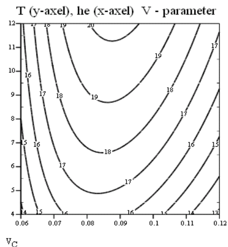
Figure 10. Tool life T [min] as a function of equivalent chip thickness h_e [mm] with chip volume V [cm³] per edge as a parameter. Insert types A, B och C.
