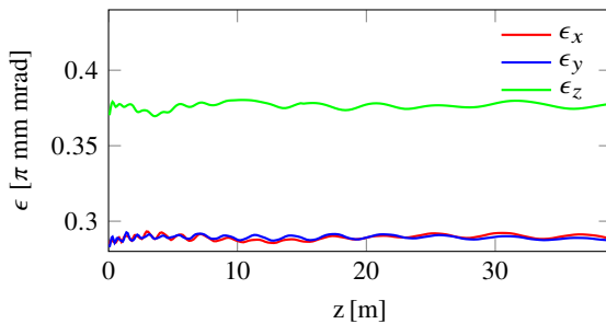
Figure 8: Emittance in x (red), y (blue) and z (green).
