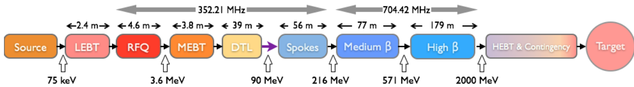
Figure 1: The overall layout of the different sections of the ESS linac. The front end including the spoke cavities run at 352.2 MHz, while the elliptical cavities run at twice that frequency. The beam energy at each intersection is given below the intersections.
