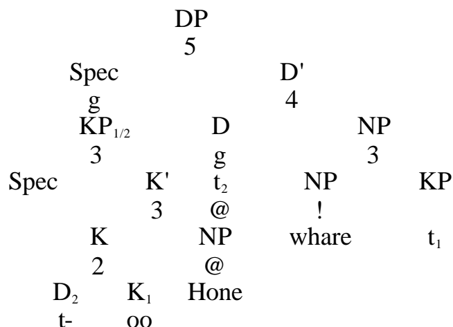
Figure 3. Incorporated possessives.
