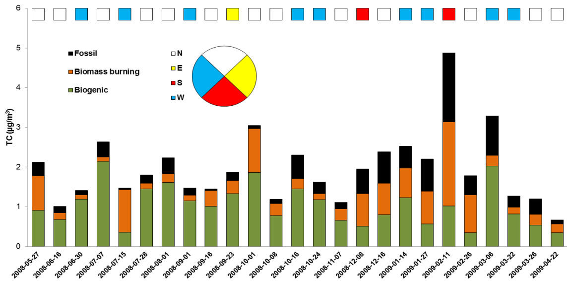
Figure 7. Apportionment of TC for all samples at Vavihill measurement station using the MCMC3 model with \delta^{13}\text{C} , Lev/EC and \text{F}^{14}\text{C} . Wind direction from trajectory analysis is showed by the top colored squares.
