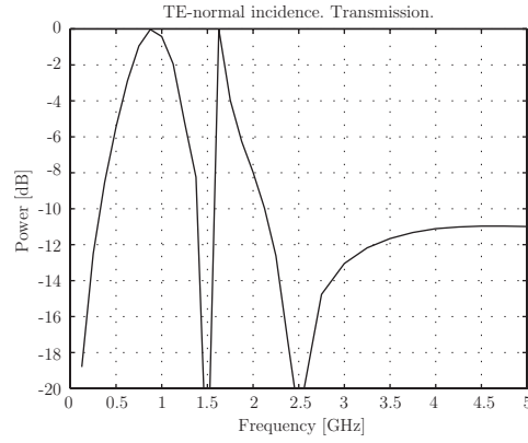
Figure 7: TE normal incidence transmission curve. Data: a = 244 mm, b = 172.5 mm, c_x = 150 mm, c_y = 1 mm, \phi_0 = 45^\circ , \epsilon_r = 5 .
