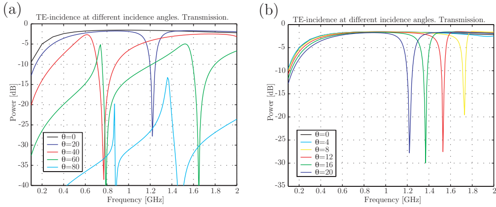
Figure 11: TE incidence transmission curve at different incident angles. (a) \theta = 0^\circ, 20^\circ, 40^\circ, 60^\circ, 80^\circ . (b) \theta = 0^\circ, 4^\circ, 8^\circ, 12^\circ, 16^\circ, 20^\circ . Data: \phi_0 = 5^\circ , \epsilon_r = 3.5 , c_x = 190 mm, a = 215 mm, and b = 172.5 mm.
