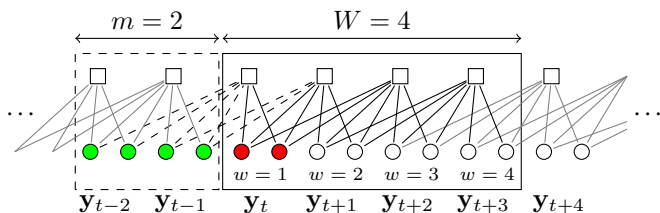
Fig. 2. Window decoder of size W = 4 at time t . The green variable nodes represent decoded blocks and the red variable nodes ( y_t ) are the target block within the current window. The dashed lines represent the read access to the m previously decoded blocks.
