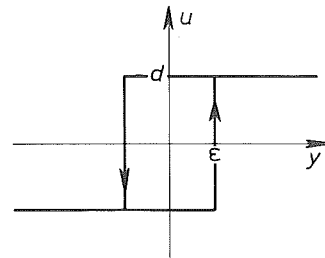
FIG. 2. Characteristics of a relay with hysteresis.
