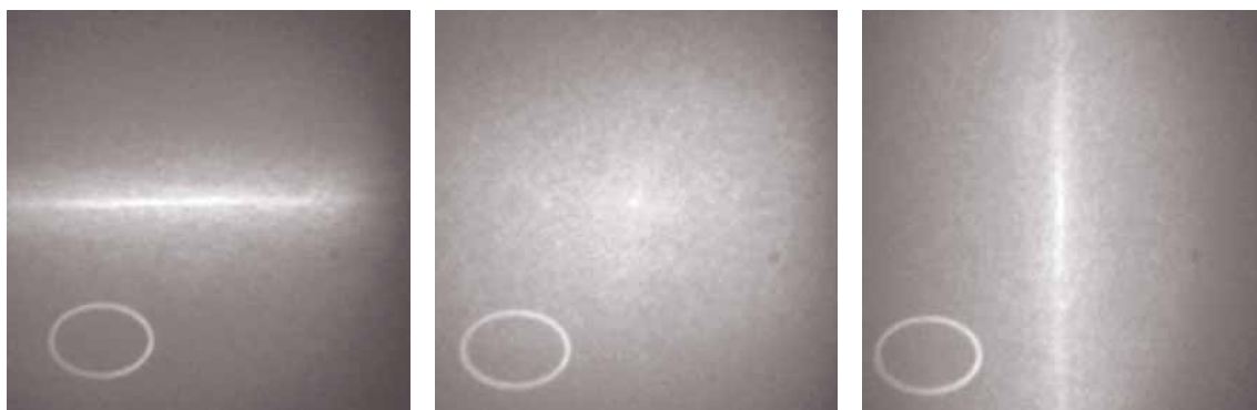
Horizontal and vertical line foci as well as the circle of least confusion from a double-pass measurement at an oblique angle.
