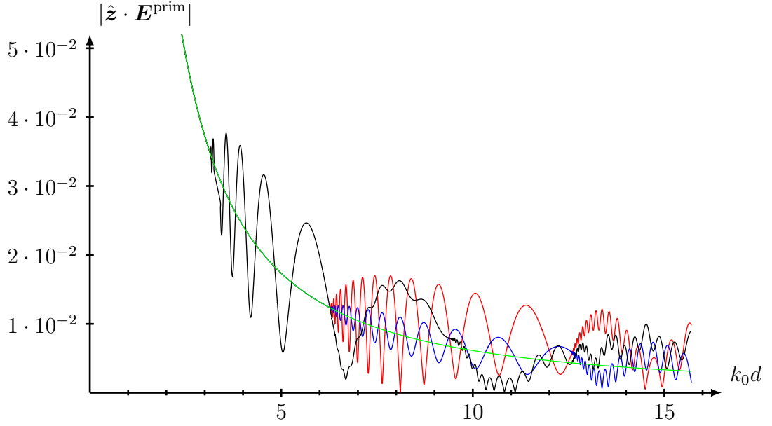
Figure 5: The absolute value of the vertical primary field, |\hat{\mathbf{z}} \cdot \mathbf{E}^{\text{prim}}(\mathbf{r})| , at a fixed point \mathbf{r} as a function of frequency, k_0 d , for a vertical electrical dipole located at \mathbf{r}_0 = -x_0 \hat{\mathbf{x}} + z_0 \hat{\mathbf{z}} , where x_0/d = 10 and z_0/d = 0 (red and blue curves), and x_0/d = 10 and z_0/d = 0.2 (black curve). The curve shows the contribution to the primary field due to the propagating modes. The locations of the planes are z_+/d = 0.5 and z_-/d = -0.5 , and the field point is \mathbf{r} = x \hat{\mathbf{x}} + z \hat{\mathbf{z}} , where x/d = 10 and z/d = 0 (red curve) and z/d = 0.3 (blue and black curves). The green curve shows the contribution of the fundamental mode alone.
