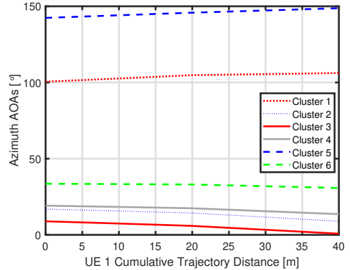
Fig. 6. Azimuth AOA with SC vs. cumulative distance of UE 1's trajectory.
