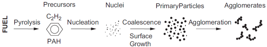
Figure 2.3: Schematic diagram of the steps in the soot formation process from gas phase to solid agglomerated particles. Reproduced from [11].
