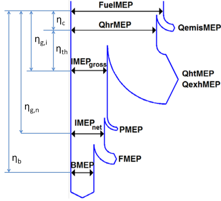
Figure 3.1: Sankey diagram of mean effective pressures
