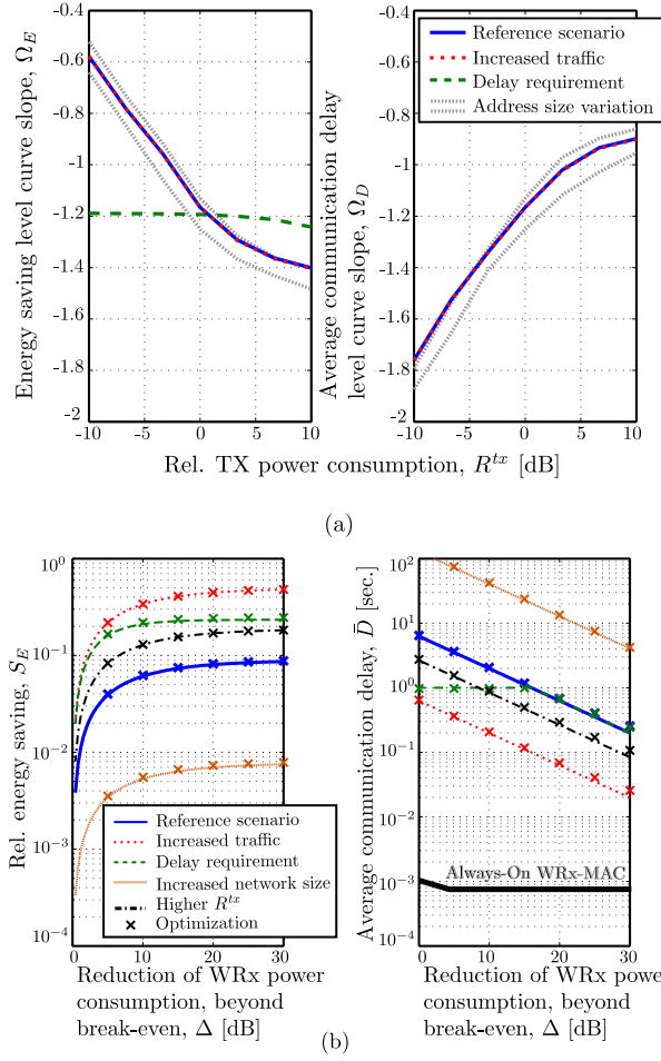
Figure 7: (a) Level curve slopes \Omega_E and \Omega_D for different relative transmit power consumptions. (b) Comparison of optimal values (crosses) and corresponding approximations (lines) of energy savings and average communication delays, for different WRx power reductions beyond break-even ( \Delta ) without implementation loss.
