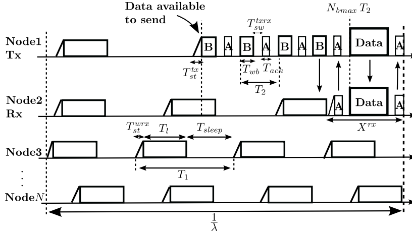
Figure 5: DCW-MAC scheme.
