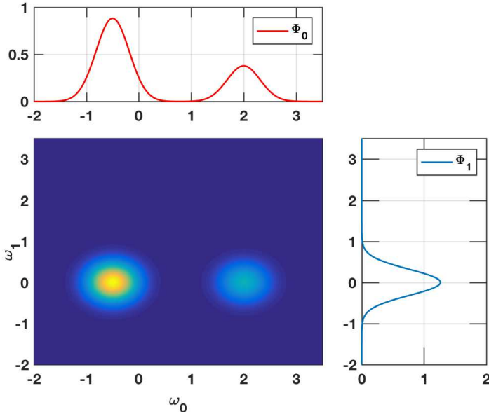
Figure 4: Two spectra, \Phi_0 , \Phi_1 , as well as a transport plan constructed as M(\omega_0, \omega_1) = \Phi_0(\omega_0)\Phi(\omega_1) .
