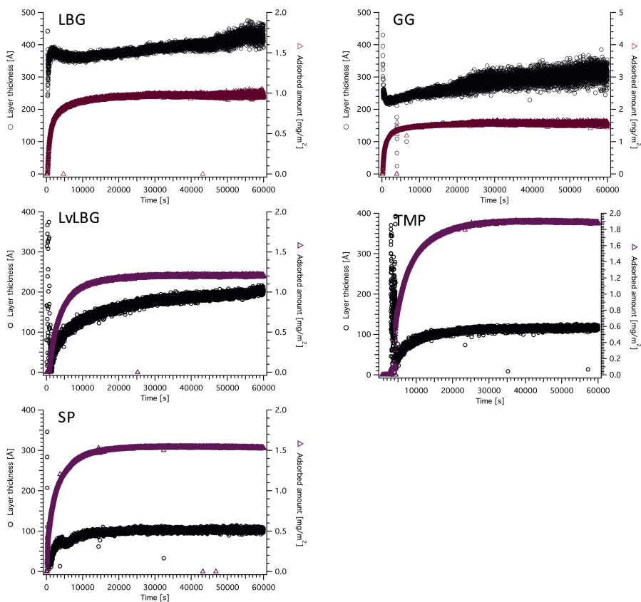
Figure S6 Mannin adsorption on hydrophobic surface measured with ellipsometry
