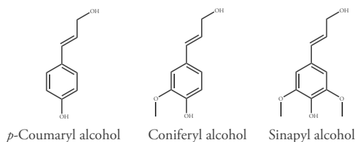
Figure 1.3 The molecular structure of the main constituents in lignin.
