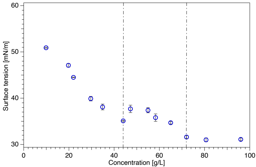
Figure 4.16 Surface tension plot of the purified hexyl manno oligoside mixture. Dash lines represent break points.
