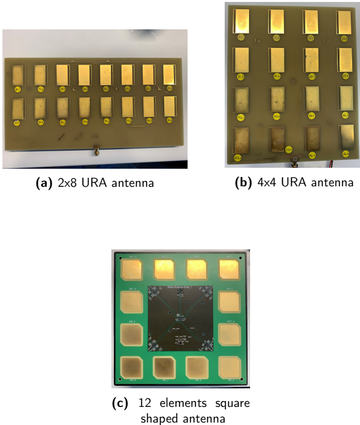
Figure 3.2: Antenna arrays
