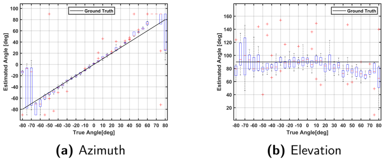
Figure 3.17: AOA estimation for 2x8 URA at Channel 38
