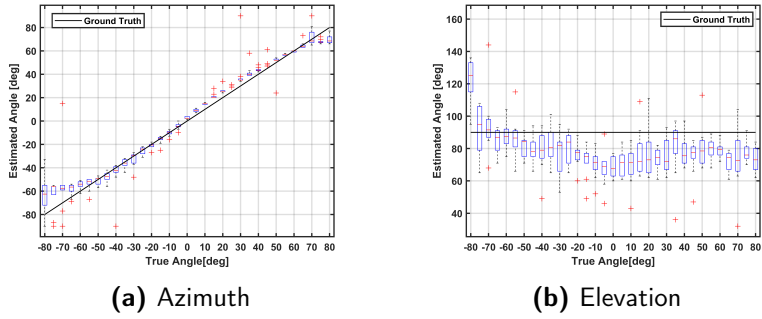
Figure 3.16: AOA estimation for 2x8 URA at Channel 37
