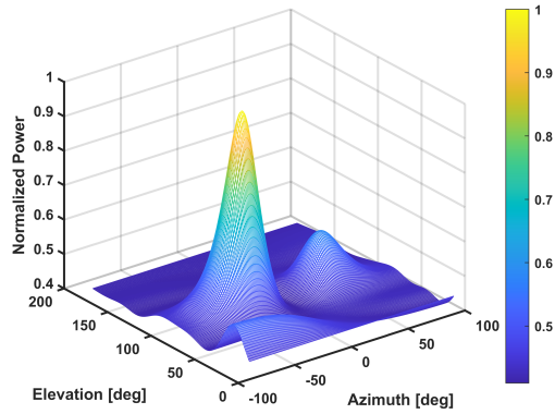
Figure 2.7: MUSIC Pseudo-Spectrum.
