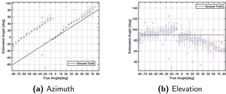
Figure 3.18: AOA estimation for 2x8 URA at Channel 39
